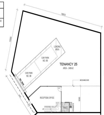
TENANCY 25 GROUND FLOOR SCALE: 1:100
