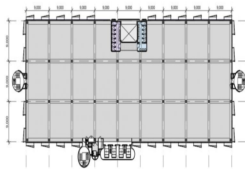
TYPICAL LEVELS 1-6
