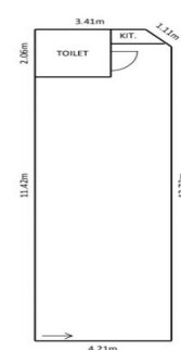
FLOOR PLAN FOR 1/1 HEIDI STREET, KULUIN QLD 4558
