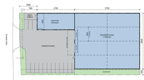
PROPOSED SITE PLAN DATE: 11/08/18
