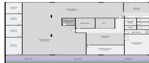
FLOOR PLAN
