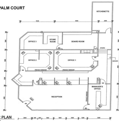
3 FLOOR PLAN
