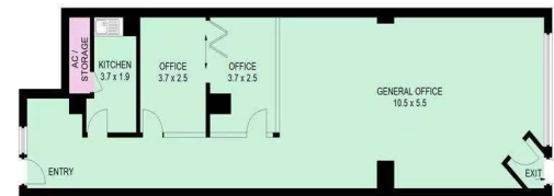
LEVEL 4 Suite 465, 311 Castlereagh Street, Haymarket This information is not to be relied upon. It is strictly for marketing & illustration purposes only. All measurements are approximate. Not to scale. No liability accepted. You must rely on your own inquiries and seek advice from your solicitor. (ID 729990)
