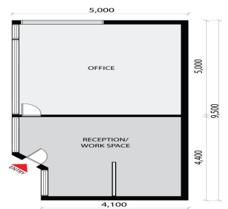
FLOOR PLAN
